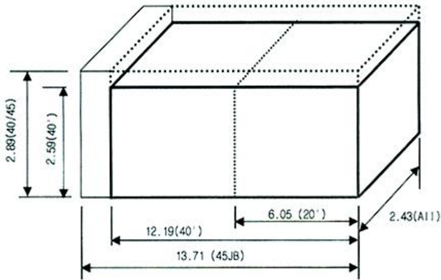
냉동 컨테이너 (Reefer Container Dimension)
